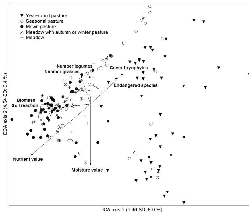
Fig. 2. DCA ordination diagram of all plots categorized by management schemes with environmental vectors as overlay ( n = 202 ). Total inertia: 6.59; for length of gradient and percentage of explained variance see axes titles.
