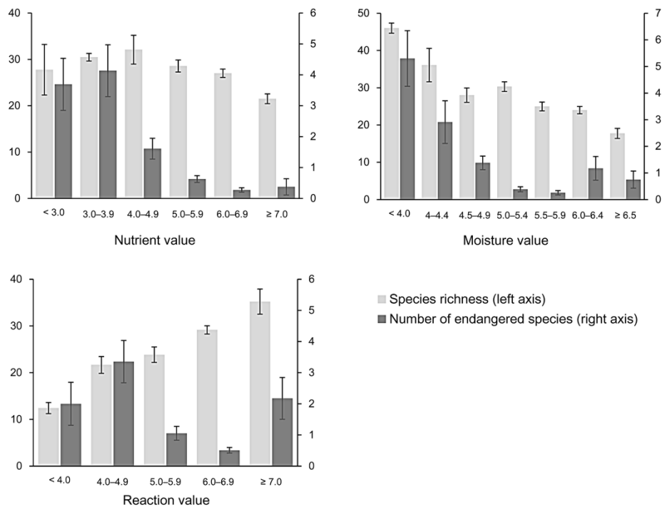
Fig. 4. Plant species richness and numbers of endangered species along gradients of nutrient supply, soil moisture and soil reaction according to Ellenberg indicator values (ELLENBERG et al. 2001). For each category of the indicator values, mean numbers of plant species and endangered species per plot are shown. All management schemes included.
