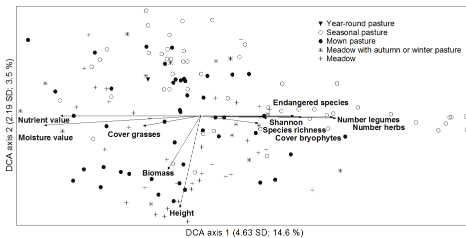
Fig. 3. DCA ordination diagram of grasslands from the three study regions Schorfheide-Chorin (northeast), Hainich-Dün (central) and Schwäbische Alb (southwest) categorized by management schemes with environmental vectors as an overlay ( n = 149 ). Total inertia: 3.63; for length of gradient and percentage of explained variance see axes titles.
